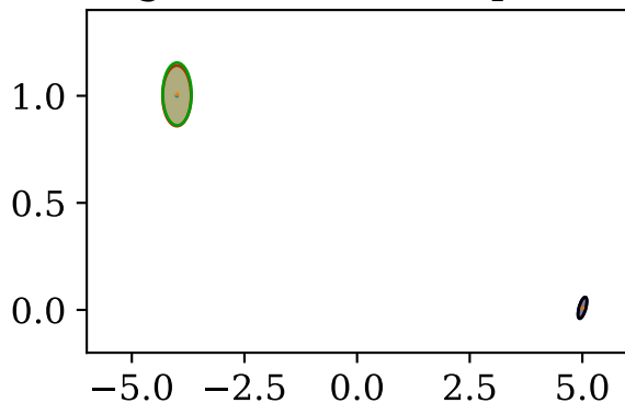
target mixture and pmc fit
