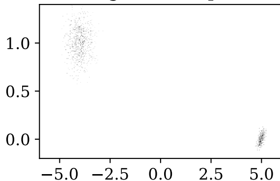
weighted samples
