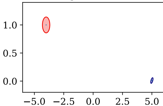
target mixture
